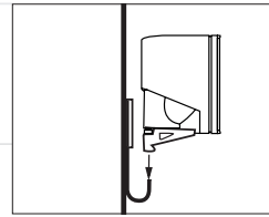
Place speaker and support on wall plate.
